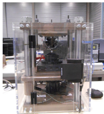
Compressibility test
